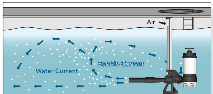
J-Ejector
